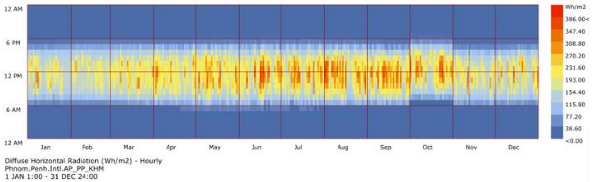
Figure 83 Heat Map of Diffuse Radiation - Phnom Penh
