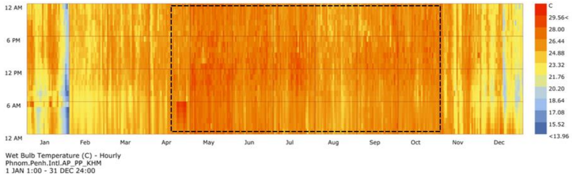
Figure 89 Heat Map of Wet Bulb Temperature - Phnom Penh
