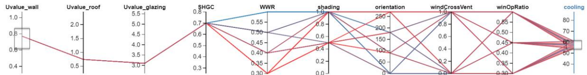
Figure 12 Results with Intermediate Envelope Configuration to Achieve High-Performance Scenario in Affordable Housing: Borey-Type
