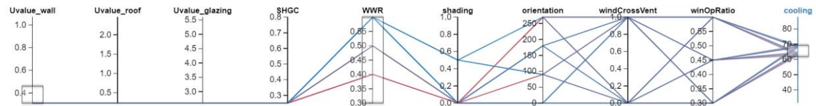
Figure 17 Results with Best-Performance Envelope Configuration to Achieve Code Compliance Scenario in Affordable Housing: Borey-Type
