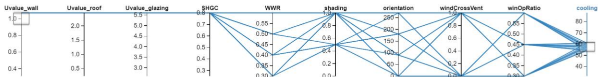
Figure 11 Results with Baseline Envelope Configuration to Achieve High-Performance Scenario in Affordable Housing: Borey-Type
