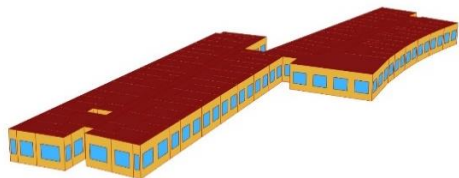
Figure 42 Building Energy Model of MHIH: Condominium-Type
