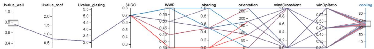
Figure 16 Results with Intermediate Envelope Configuration to Achieve Code Compliance Scenario in Affordable Housing: Borey-Type
