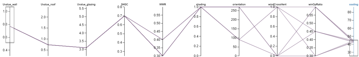
Figure 22 Results with Baseline & Intermediate Envelope Configurations to Achieve Near-Zero Scenario in Affordable Housing: Condominium
